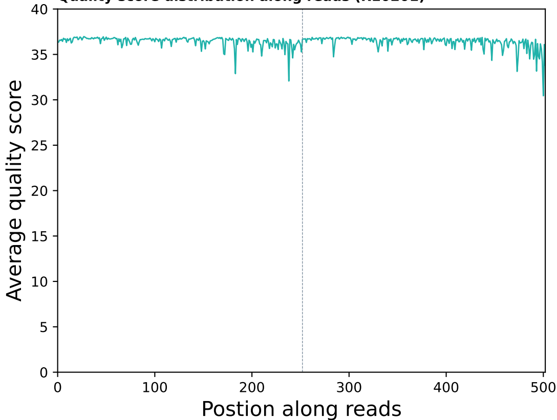
Quality score distribution along reads (R10201)
